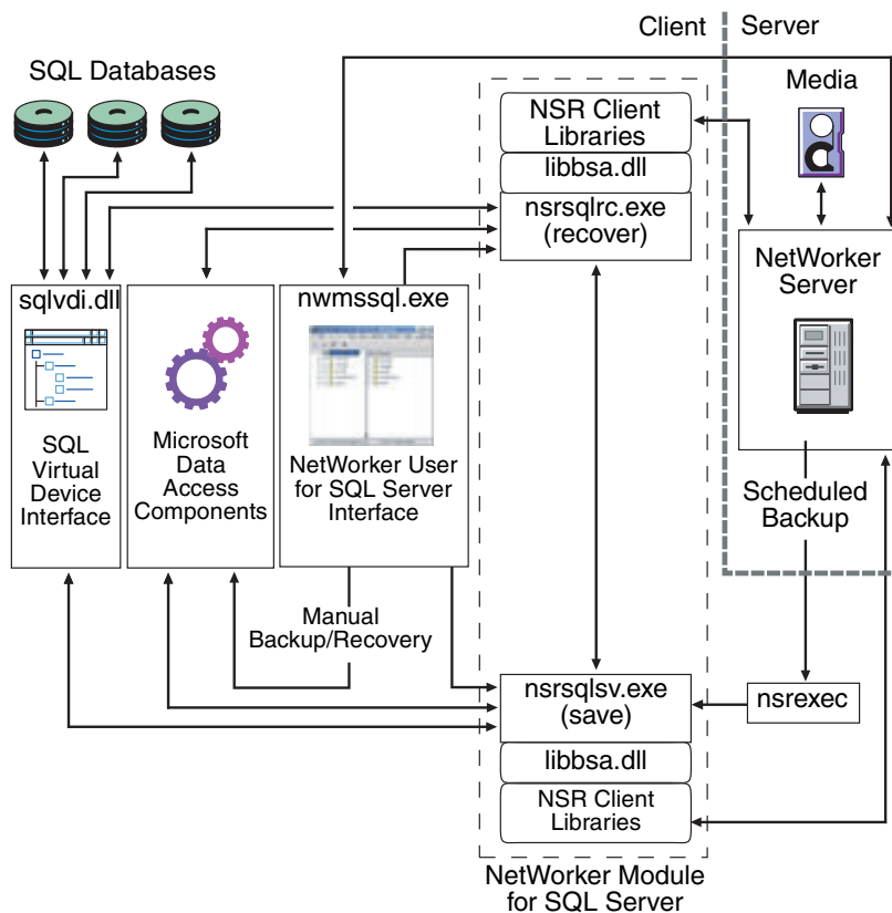
Figure 1 Module and NetWorker Setup with SQL Server
