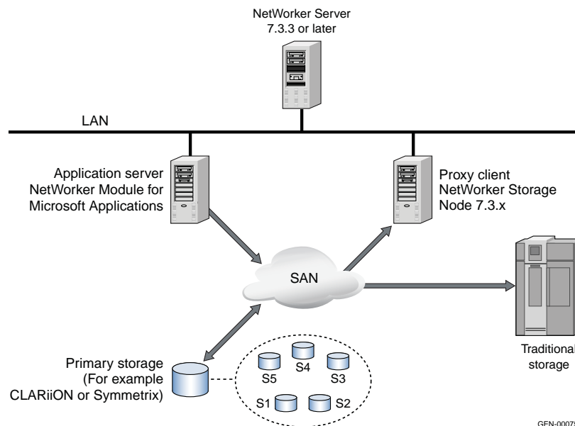
Figure 3 LAN-free configuration
